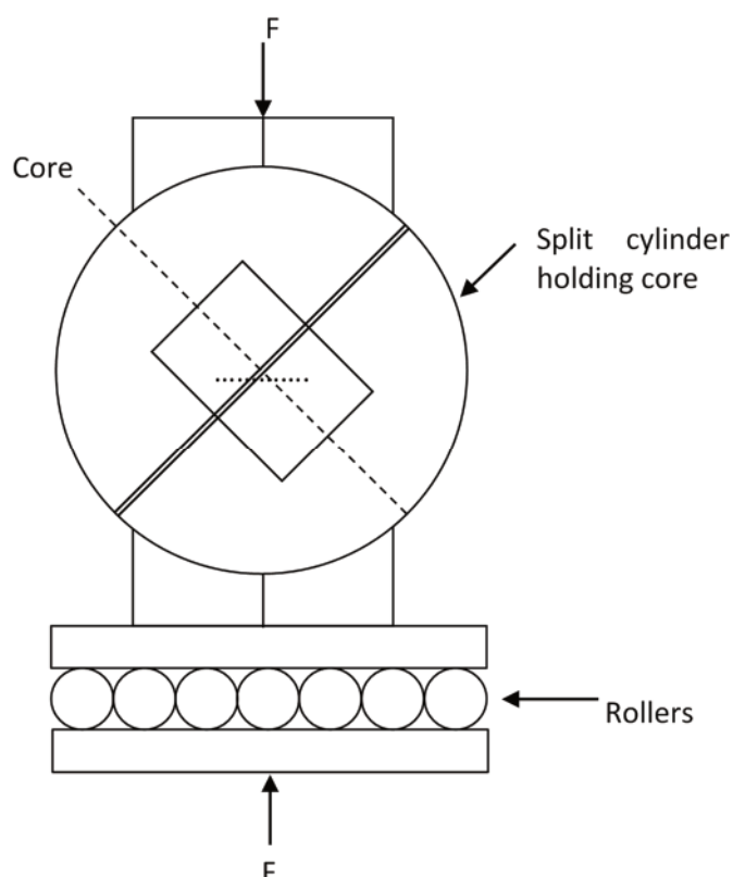
Figure 15 Schematic diagram of modified GOST shear test
